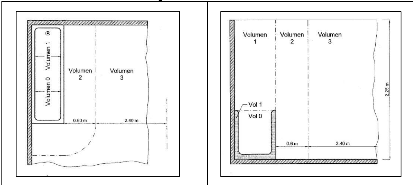
Figura 11.6.1 – BAÑERA
